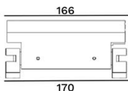
Asymmetric Louver
